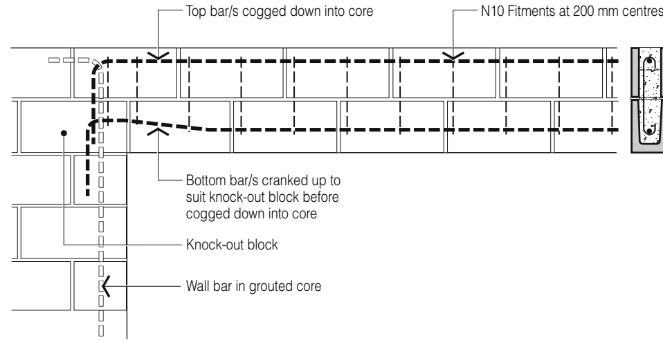
SIMPLY-SUPPORTED LINTEL
